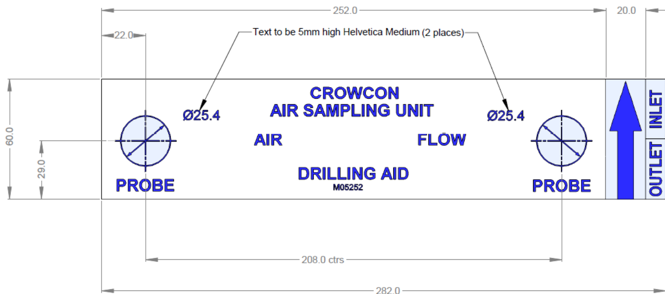
Drilling Template Label Dimensions
